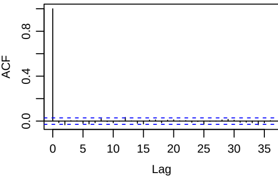
ACF Standardized Residuals
